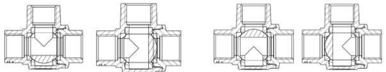
S.73 3-WAY "T" PORT OPERATING POSITIONS
