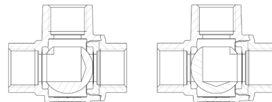
S.76 3-WAY "L" PORT OPERATING POSITIONS
