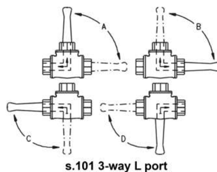
s.101 3-way L port
