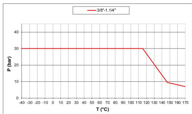
Pressure-temperature chart
